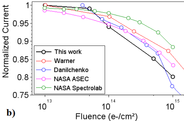
Fig. 3. a) J - V characteristics of GaAs G1 cell under AM0 light at 25°C and for different fluences b) Degradation of the photocurrent for G1 as a function of fluence, compared to literature data [15],16]
