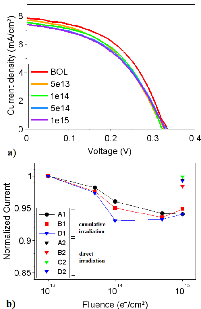
Fig. 5. a) J - V characteristics of InGaAsN A1 cell under AM0 > 870 nm light at 25°C and for different fluences b) Degradation of the photocurrent in InGaAsN cells as a function of fluence
