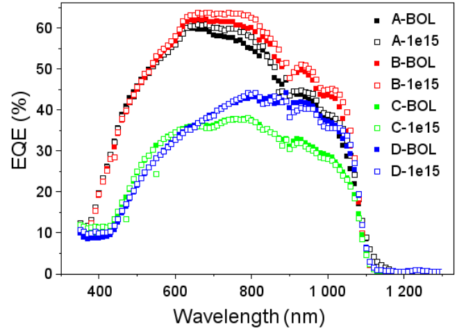
Fig. 6. EQE before and after 1 MeV electrons irradiation for 4 InGaAsN cells A, B, C and D
