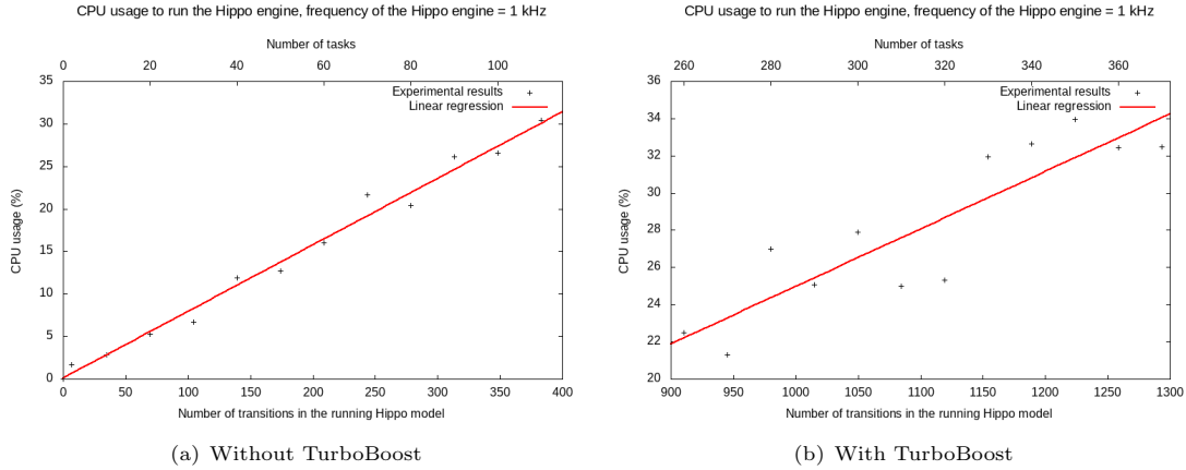
Figure 7: CPU usage as a function of number of HIPPO tasks.
