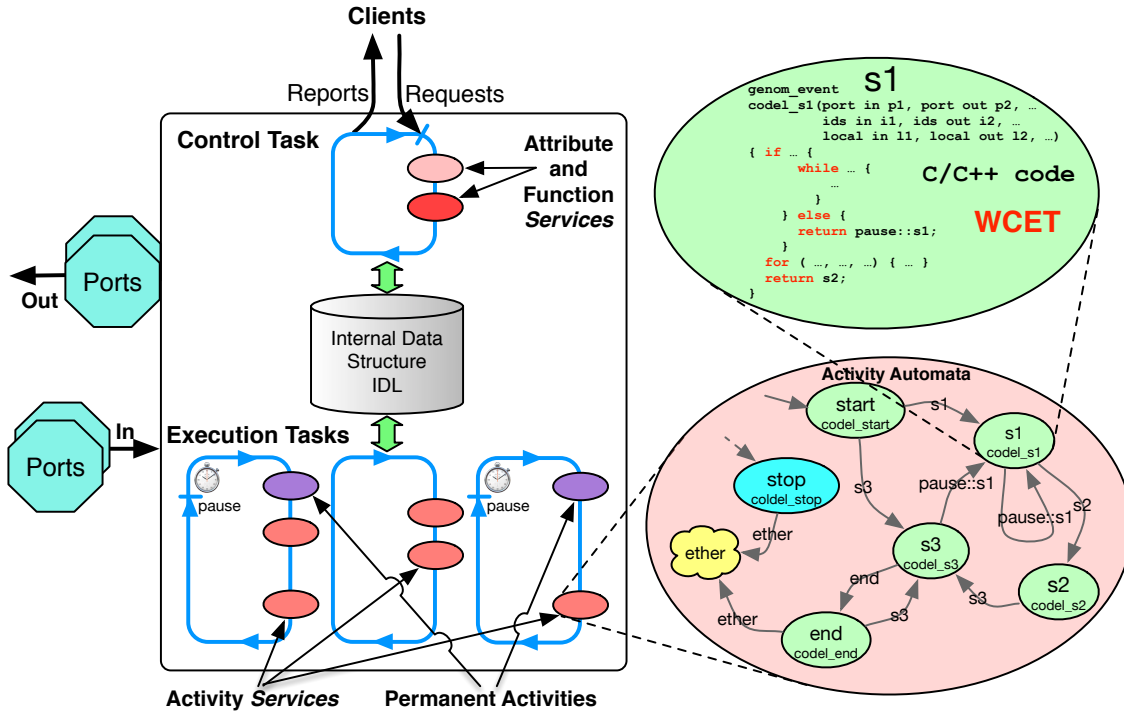
Figure 10: A G^{\text{en}}\text{M} generic functional component (module).
