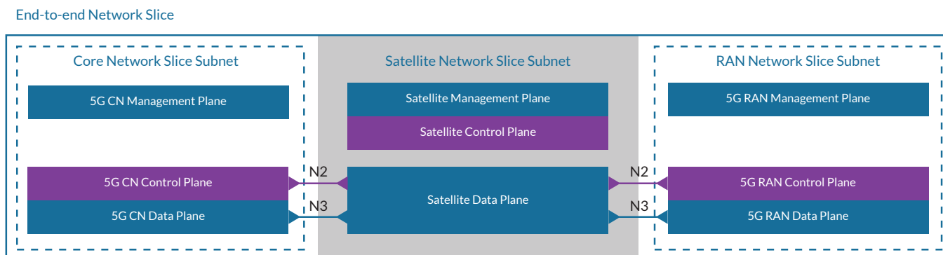
FIGURE 12 Network Slice Plane Interconnection
