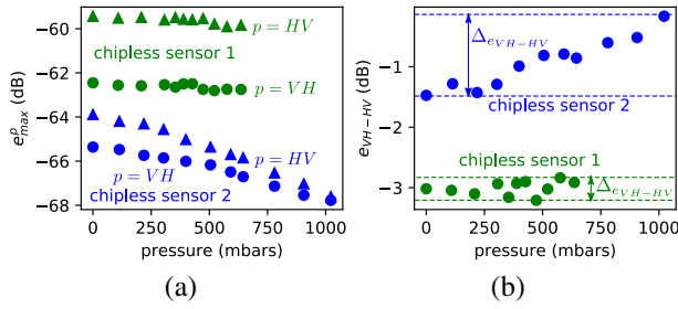
Figure 4. (a) Estimator e_{max}^p in function of the applied pressure of the chipless pressure sensors 1 (in green color) and 2 (in blue color) for p = VH (circles) and p = HV (triangles). (b) Identification parameter e_{VH-HV} in function of the applied pressure of the chipless pressure sensors 1 (in green color) and 2 (in blue color).
