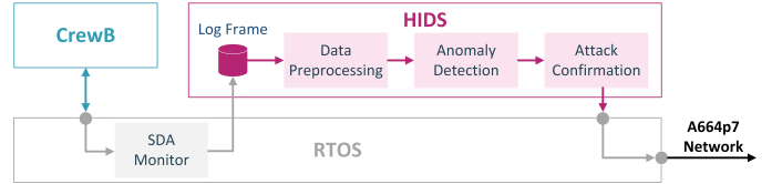
Figure 7: Architecture of the Embedded Prototype
