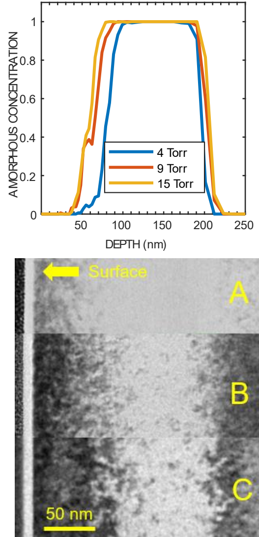
Fig. 3: (Top) Simulation of amorphous concentration as function of the depth for a 60 keV carbon implantation with a dose of 1.5 \cdot 10^{15} \text{ cm}^{-2} and for cooling pressures of 15, 9 and 4 Torr. (Bottom) A, B and C are the TEM images of 60 keV carbon implanted wafers with a dose of 1.5 \cdot 10^{15} \text{ cm}^{-2} and a cooling pressure of 15, 9 and 4 Torr respectively.
