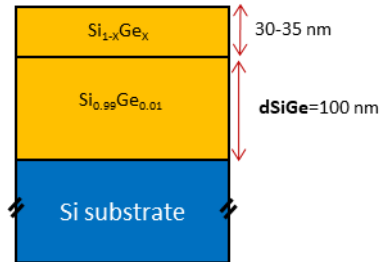
Fig. 2: Corresponding modeling for 1D numerical simulations with LIAB tool.
