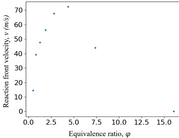
Figure 4. Simulation of the reaction front velocity of 4.5 \mu\text{m} thick Al/CuO multilayers as a function of the equivalence ratio, \phi . The Al/CuO bilayer thickness is fixed at 300 nm, and T_{max} = 2843 K.
