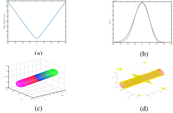
Fig. 2: (a) Miss distance (m.) (b) Instantaneous probability of collision \mathcal{P}(t) with (blue) or without velocity uncertainties (red) at TCA (c) 3D Swept-volume shape (no velocity uncertainty) (d) PSS approximation of degree d = 4 .
