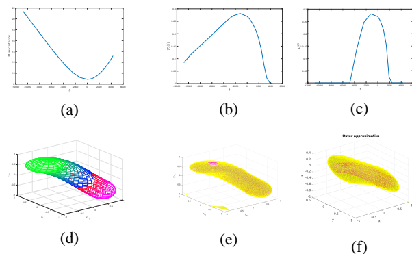
Fig. 3: (a) Miss distance (m) (b) Instantaneous collision probability \mathcal{P}(t) with (c) and without (d) velocity uncertainty (d) 3D Swept-volume shape (no velocity uncertainty) (e) PSS approximation d = 8 (f) Projection of 6D PSS approx, d = 8 , for a fixed mean velocity.
