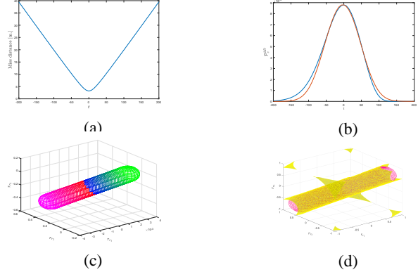
Fig. 2: (a) Miss distance (m.) (b) Instantaneous probability of collision \mathcal{P}(t) with (blue) or without velocity uncertainties (red) at TCA (c) 3D Swept-volume shape (no velocity uncertainty) (d) PSS approximation of degree d = 4 .
