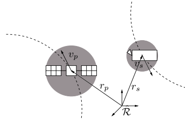
Fig. 1: Encounter between two spherical objects.
