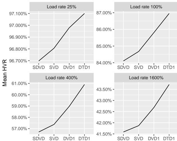
Figure 5: Mean Hit Value Ratio performed by different online algorithms over 1000 scenarios for each load rate.
