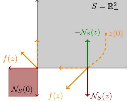
FIGURE 2. State trajectories in constrained system with S = \mathbb{R}_+^2 .
