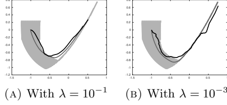
FIGURE 6. For two values of regularization parameter \lambda , we represent in dark gray the empirical first moments of the trajectory of (36) (obtained by sampling initial conditions) and in black the first pseudo-moments of the terminal measure computed with Glopti-Poly and MOSEK for the relaxation of order 4 (moment-SOS of degree 8). In light gray we represent for reference the ensemble trajectories for a uniform distribution of the initial condition in the box S(0) .
