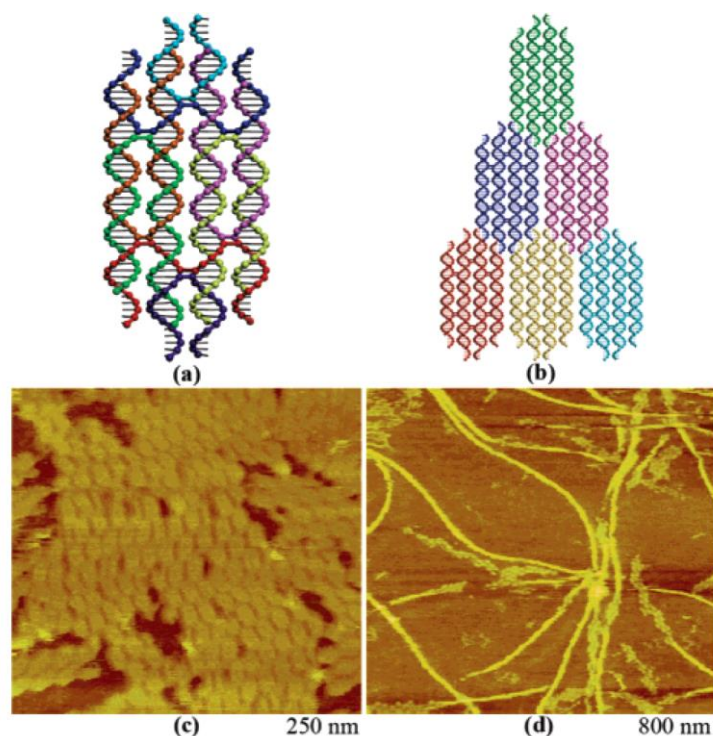
Figure 3: double-double crossover (DDX) DNA-based structure (top schematics) and AFM image of a 2D crystal made of branched DDX motifs (lower view). (Reprinted with permission from J Am Chem Soc 2005, 127 (50), 17590-17591. Copyright (2005) American Chemical Society)
