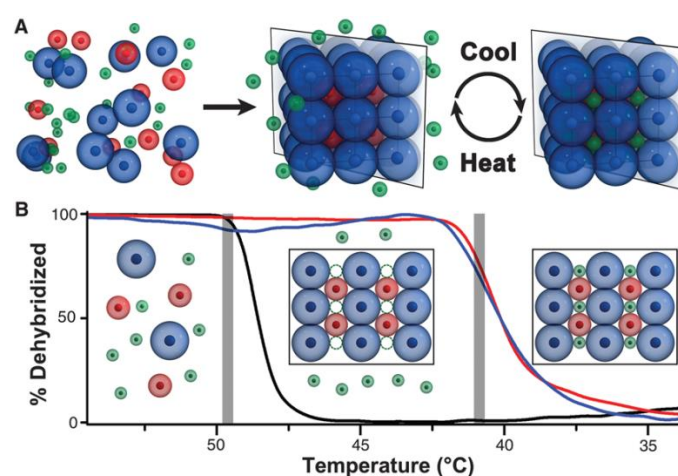
Figure 12: Diagram of the self-assembly of nanoparticles by DNA in ternary crystalline structures. A binary structure is first synthesized prior to insertion of a third size nanoparticles into a predetermined site (A). In (B), the thermal analysis of the ternary structure is presented. (Reprinted with permission from Science 2013, 341 (6151), 1222-1225, Copyright (2013), Science American Association for the Advance of Science)
