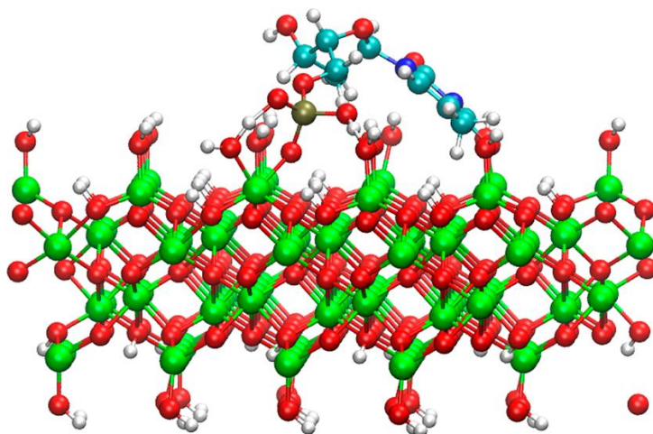
Figure 16: Chemisorption of dTMP on a hydrated \text{Al}_2\text{O}_3 surface (with an -\text{OH} termination) in the most stable case, i.e. with formation of covalent bonds at the level of phosphate and thymine groups. 100
