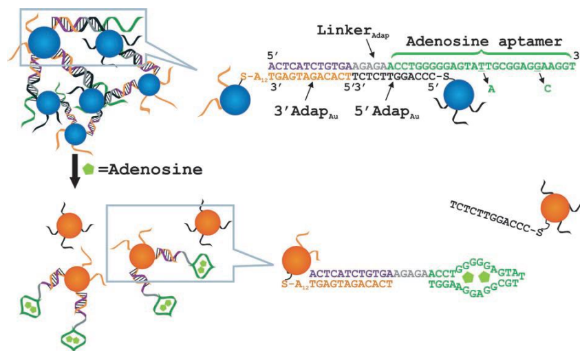
Figure 13: Schematic diagram of the detection of adenosine using the colorimetric method.
