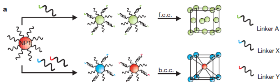
Figure 8: Diagram summarizing the influence of the linker on the crystalline structure obtained after the self-assembly of gold nanoparticles. (Reprinted with permission from Nature 2008, 451 (7178), 553-556, Copyright (2008), Springer Nature)
