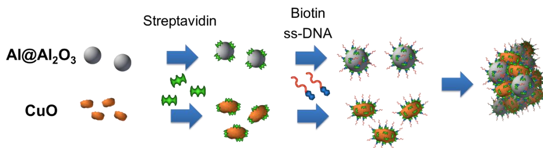
Figure 13. Illustration of the functionalization process developed to enable the DNA-directed self-assembly of core-shell Al (Al covered with Al 2 O 3 shell) and CuO nanoparticles.
