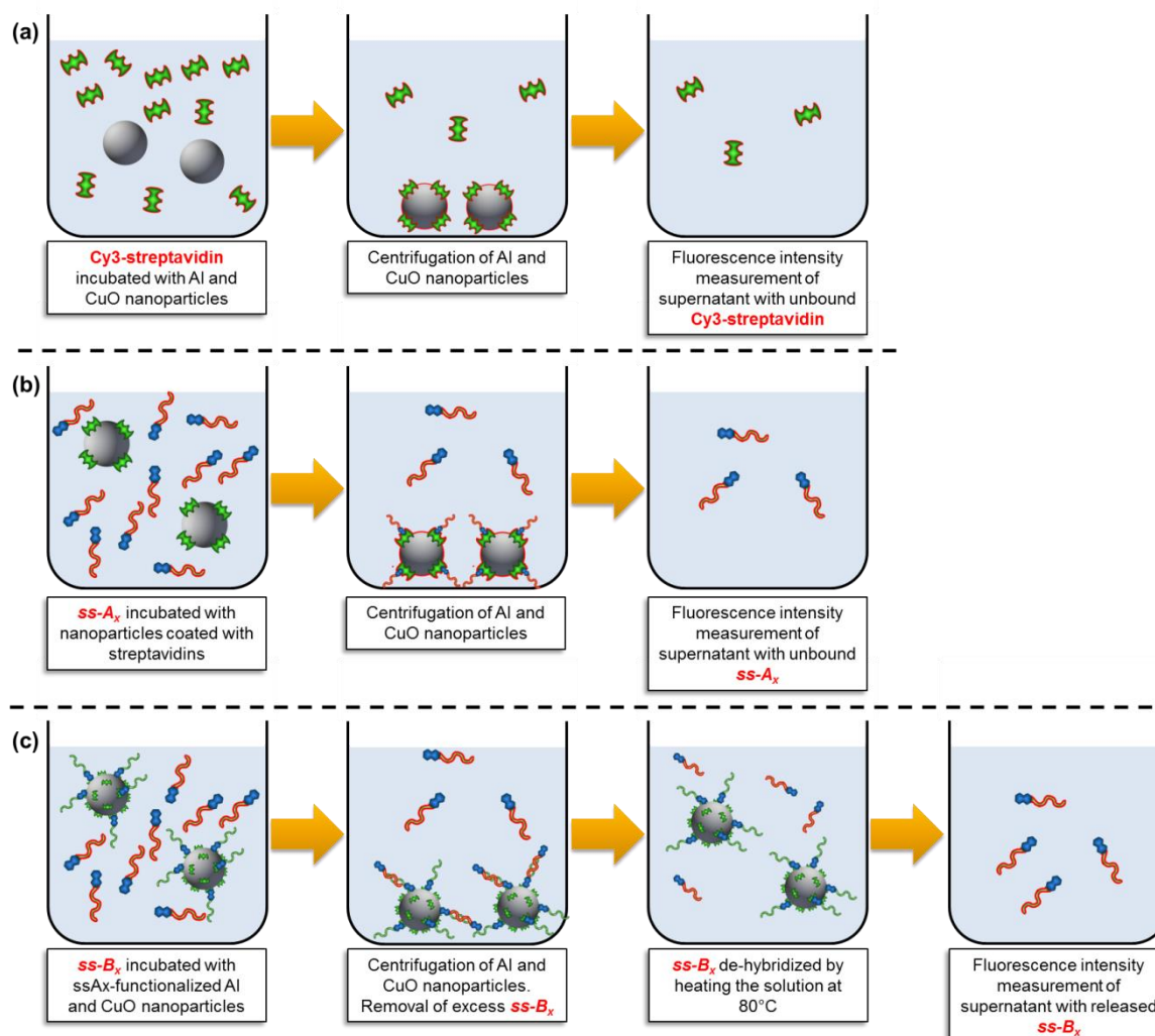
Figure 20. Schematic representation of the process developed for the determination of (a) streptavidin surface density on CuO or Al nanoparticles, (b) the DNA surface density on CuO or Al nanoparticles and (c) the hybridization efficiency on CuO or Al nanoparticles.
