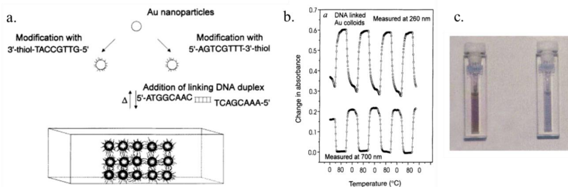
Figure 5: (a) Schematic diagram of the linker self-assembly of 13-nm diameter gold nanoparticles (left figure). (b) Measuring the absorbance at 260 and 700 nm of the colloidal solution of nanoparticles as a function of temperature (0 and 80 °C) and demonstrating the reversibility of the hybridization of the DNA strands. (c) Image of the colloidal solution heated to 80 °C (red), and cooled to 0 °C (blue). (Reprinted with permission from Nature 1996, 382 (6592), 607-609, Copyright (1996), Springer Nature)
