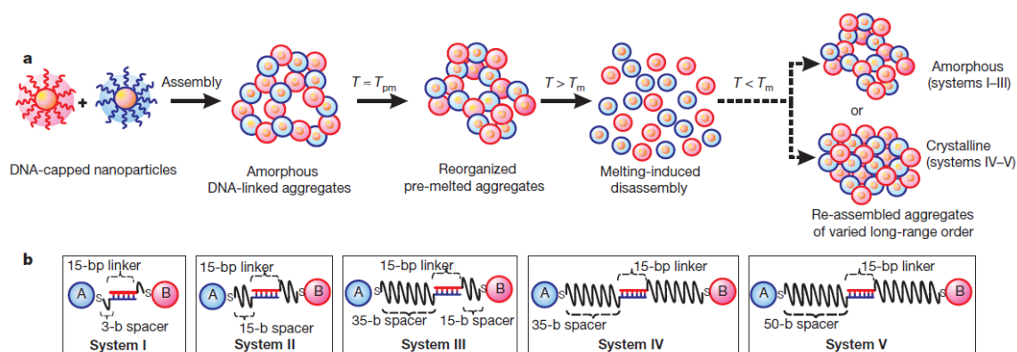
Figure 10: Diagram showing the behaviour of nanoparticle aggregates formed upon DNA self-assembly versus temperature and the length of DNA strands used. (Reprinted with permission from Nature 2008, 451 (7178), 549-552, Copyright (2008), Springer Nature)
