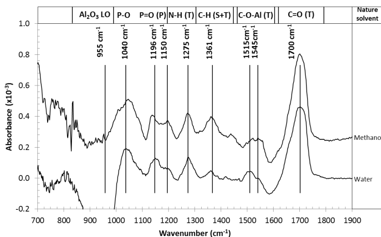
Figure 18: Influence of the nature of the solvent on the IR absorbance spectra of an alumina surface after dTMP deposition. The incubation of the surface was performed using methanol (top curve) and water (bottom curve) with the same concentration of dTMP to a clean alumina substrate in both cases. Related dTMP regions are reported on the top of the figure: T for thymine, S for sugar, and P for phosphate according to assignments resulting from DFT calculations. 100
