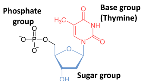
Figure 15. Schematic of the dTMP molecule with its subunits equivalent to those of DNA.
