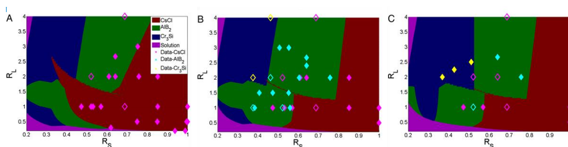
Figure 9: Gold nanoparticle phase diagrams as a function of nanoparticle size ( R_S ) or linker length ( R_L ) for three different stoichiometries (in a binary mixture, the ratio in terms of the population of nanoparticles functionalized with a given sequence versus another set of nanoparticles with the complementary sequence): (A) 1:1, (B) 2:1, (C) 3:1. The symbols represent the experimental points: the solid symbols represent the pure structures, while the voids represent polymorphic structures. Overall, there is good agreement between experimental points and theoretical results. 47
