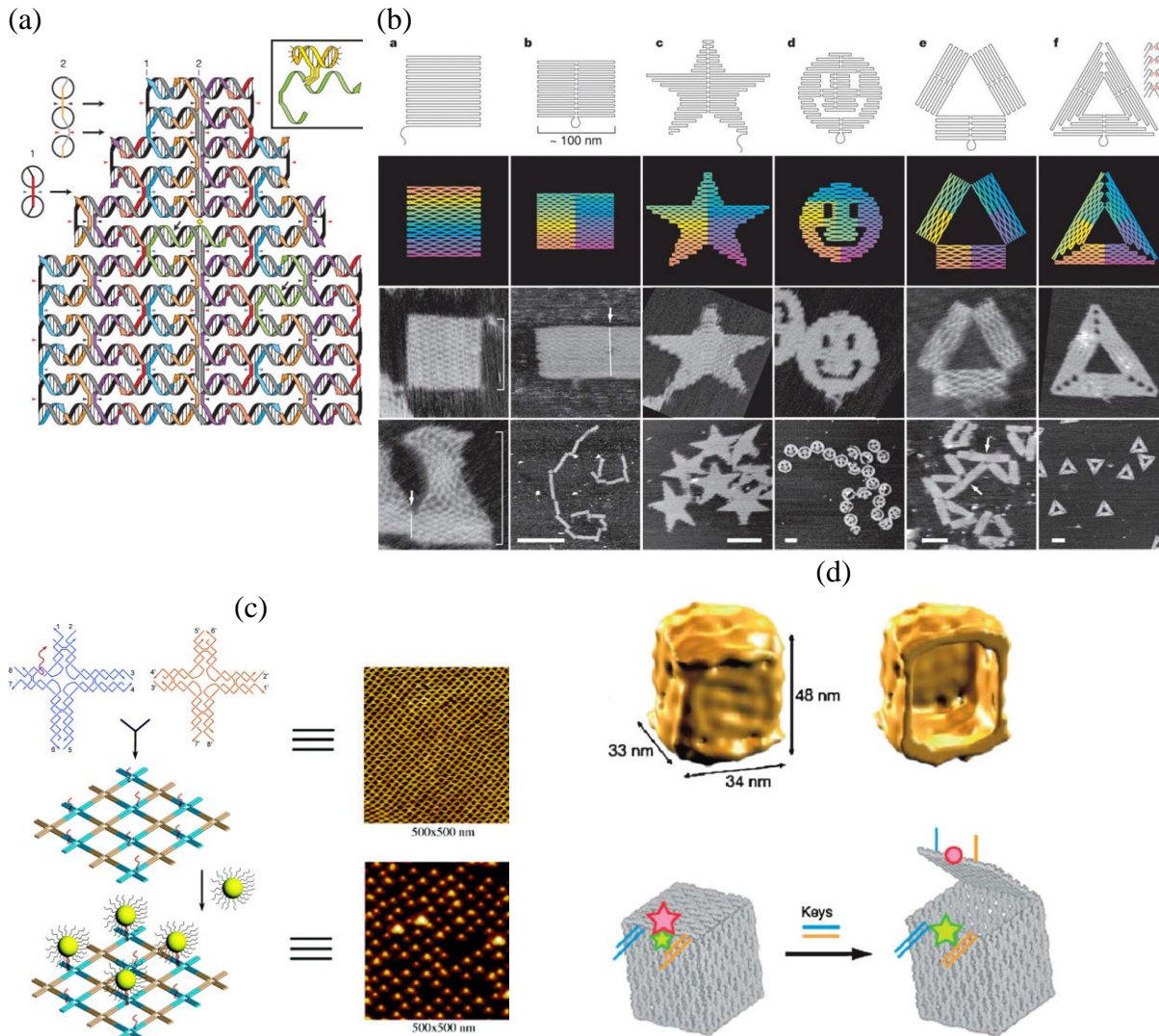
Figure 4: (a) Design of a DNA origami. (b) Different shapes obtained using the origami technique: a, square; b, rectangle; c, star; d, smiley; e and f, triangles. The first two lines correspond to design images from computer simulation, while the two other lines correspond to experimental validations. (Reprinted with permission from Nature 2006, 440 (7082), 297-302, Copyright (2006), Springer Nature); (c) DNA nanostructures used as templates for the assembly of a 2D network of gold nanoparticles. (Reprinted with permission from Nano Lett 2006, 6 (2), 248-251, Copyright (2006), American Chemical Society) (d) Full origami DNA box. The box may be actuated for closing/opening through the introduction of an oligonucleotide (the top image reconstructed from transmission electron cryomicroscopy experiment, and the bottom image is a schematic of the origami box. (Reprinted with permission from Nature 2009, 459 (7243), Copyright (2009), Springer Nature)
