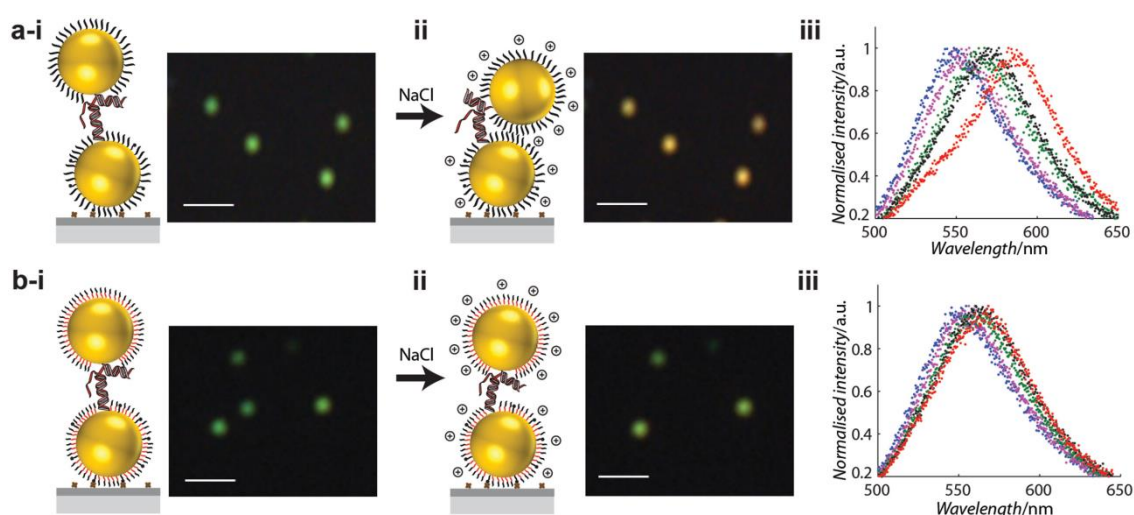
Figure 11: Comparison of the variation in the interparticle distance of 40-nm diameter gold nanoparticles organized into dimers according to the use of hydrophilic (a) or amphiphilic (b) ligands for their stabilization after increases in the saline concentration (i: 5 mM NaCl; ii: 800 mM NaCl) by dark field microscopy and spectral absorbance analysis. (Reprinted with permission from Small 2015, 11 (42), 5696-5704, Copyright (2015), Wiley)
