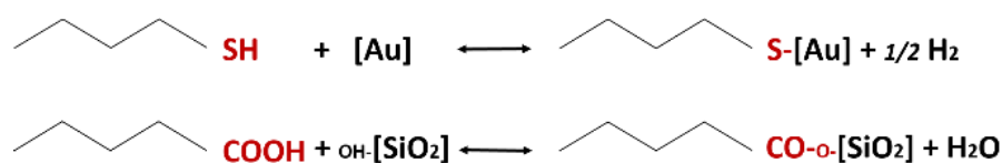
Figure 6: Typical thiol-terminated species for a gold surface (in brackets) chemical reaction (top chemical reaction equation) and carboxylic acid (COOH)-terminated species to a hydroxylated (OH) silicon dioxide surface (in brackets) chemical reaction (bottom equation).
