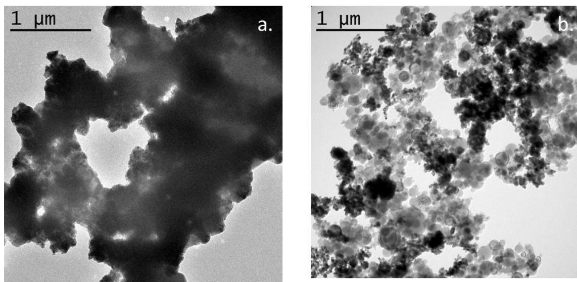
Figure 24: TEM images of nanocomposites made by direct mixing of Al and CuO nanoparticles (a), and assembled with optimized and complementary DNA strands (b).
