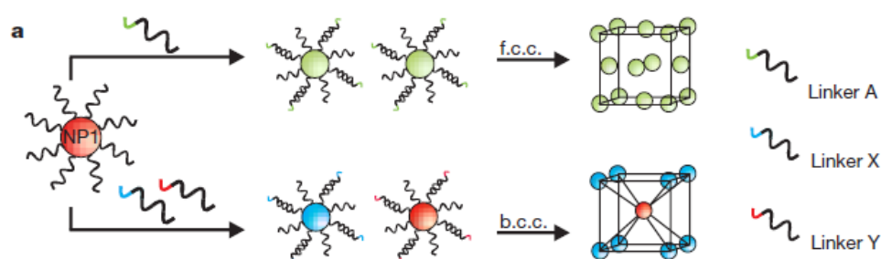
Figure 8: Diagram summarizing the influence of the linker on the crystalline structure obtained after the self-assembly of gold nanoparticles. (Reprinted with permission from Nature 2008, 451 (7178), 553-556, Copyright (2008), Springer Nature)
