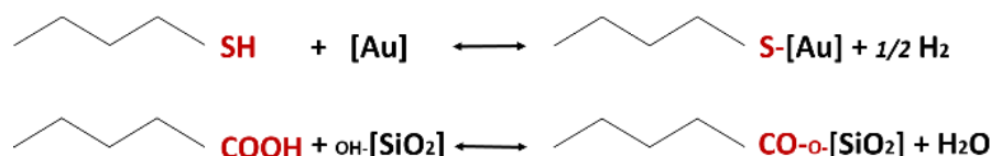
Figure 6: Typical thiol-terminated species for a gold surface (in brackets) chemical reaction (top chemical reaction equation) and carboxylic acid (COOH)-terminated species to a hydroxylated (OH) silicon dioxide surface (in brackets) chemical reaction (bottom equation).
