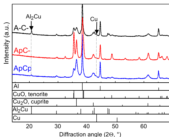
Figure 6. XRD patterns of ARM-prepared 8Al:3CuO thermite powders quenched from 650 K. The strongest peaks of \text{Al}_2\text{Cu} and Cu are indicated with arrows.
