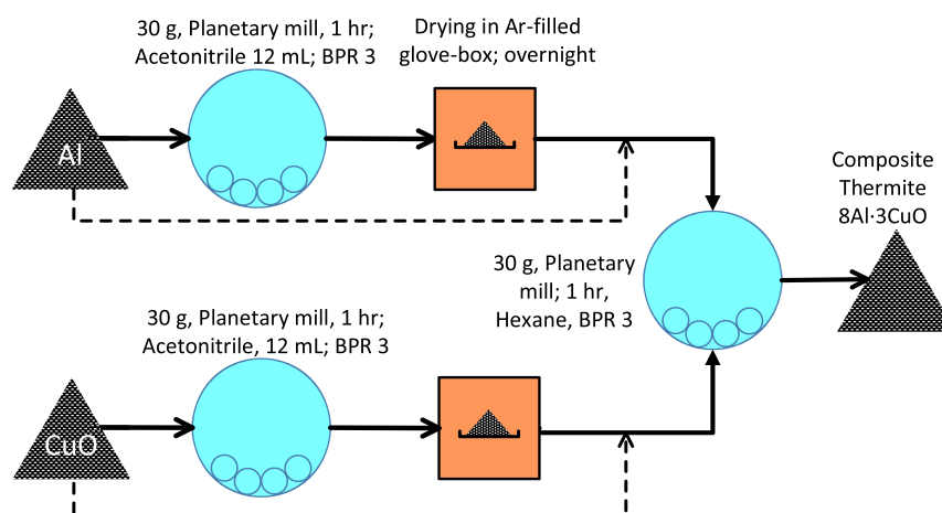
Figure 2. Two-stage milling procedure used to prepare nanocomposite thermite powders with premilled Al and/or CuO.
