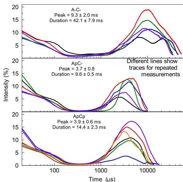
Figure 4. Integrated time-resolved emission traces obtained by processing the high-speed video frames for different powders A-C-, ApC-, and ApCp.
