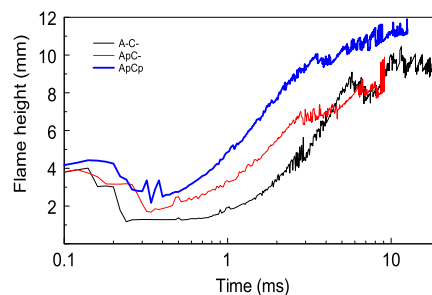
Figure 5. Time-resolved flame height profiles of A-C-, ApC-, and ApCp powder combustion by ESD. Each profile was average among at least five repetitions.
