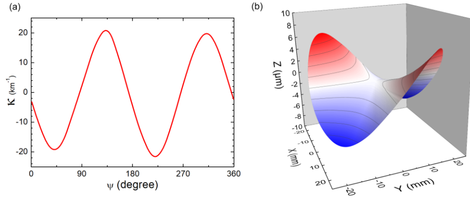
Figure 3. The curvature measured on a bare 50 mm diameter, 350 \mu\text{m} thick GaAs (001) oriented wafer while rotating at 12 rpm around its axis, at 580°C (a) allows for its complete shape reconstruction in real-time (b).
