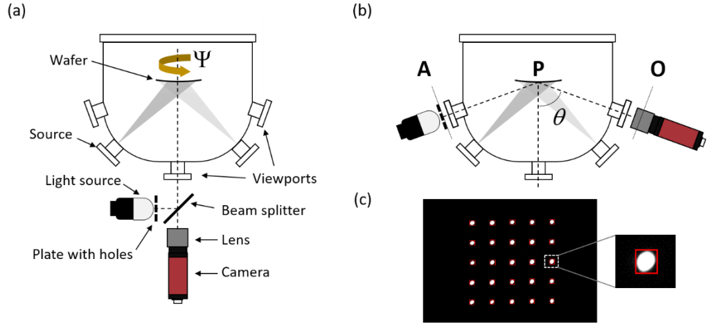
Figure 1. Experimental configuration of the MIC system mounted on a MBE chamber in order to measure the curvature of a wafer in situ and in real-time during MBE growth ((a) and (b)). The system can be mounted either in normal incidence (a) or in tilted specular reflection incidence (b). The position of the object plane (A), the pole of the reflecting surface (P), and the focal plane of the objective lens (O) are noted in (b). (c) shows a typical virtual image of a 1.6\times 1.6 \text{cm}^2 object captured with the camera, where our software tracks the positions of luminous spots forming a 5\times 5 matrix (red rectangles).
