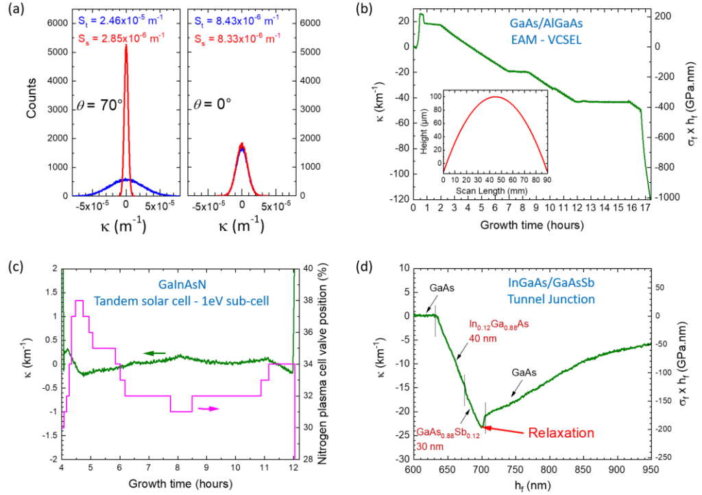
Figure 4. (a) Measurement of the curvature \kappa in tangential (blue) and sagittal (red) planes of a flat mirror repeated 10^5 times, and mounted on an optical vibration-free bench in order to get insights on the precision of our MIC-based tool. The distances \overline{OP} and \overline{AP} are those of the configuration in our MBE412 system (0.516 m and 0.678 m respectively). The incidence angle is either \theta = 70^\circ (left) or \theta = 0^\circ (right). The object is composed of a 1.6 \times 1.6 \text{ cm}^2 , 5 \times 5 matrix of luminous spots. (b)(c)(d) In situ measurements of the curvature change during MBE growths. (b) Complete growth of a \sim 10 \mu\text{m} thick, 17 hours long GaAs/AlGaAs EAM-VCSEL. The insert is the height scan of the grown structure with respect of the bare wafer measured by a P15+ KLA Tencor. (c) Focus on the controlled growth of the 1eV GaInAsN sub-cell alloy of a tandem solar cell. The variation of the opening of the nitrogen plasma cell valve is shown in pink (right scale). (d) Focus on a InGaAs/GaAsSb tunnel junction where a strain relaxation is observed when the total structure grown thickness is \sim 700 nm.
