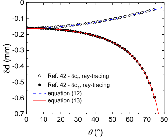
Figure 5. Laser deflectometry spots spacing change ( \delta d ) versus incidence angle \theta on a convex surface ( R = -10 m): comparison between ray-tracing simulations made in reference (42) (open and plain circles in tangential and sagittal planes respectively) and equations (12) and (13) (blue dash and red continuous curves respectively) with the parameters set in reference (38) ( L = 0.8 m, d = 1 m)
