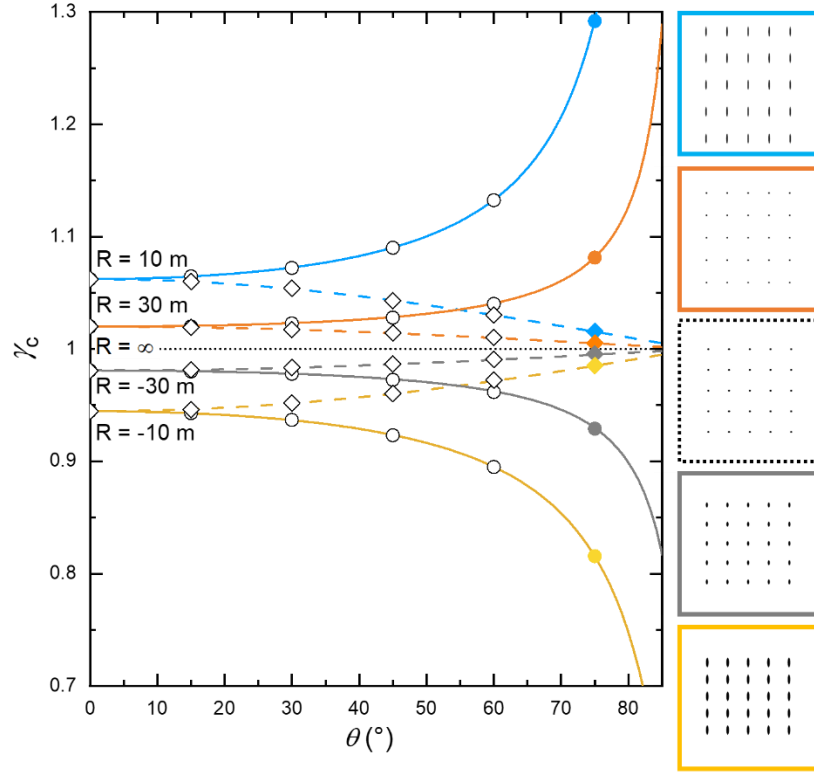
Figure 2. Captured magnification \gamma_c calculated (curves) and extracted (points) by our image analysis algorithm out of images simulated with Zemax OpticStudio ® as a function of tilt angle \theta and for radii of curvature of 10 m (blue), 30 m (orange), infinite (dotted dark), -30 m (grey) and -10 m (yellow). The distances \overline{OP} and \overline{AP} used for calculation and simulation are those of our MBE 412 system's configuration (0.516 m and 0.678 m respectively). The curves show calculation in sagittal (solid) and tangential (dash) directions thanks to equations (6) and (7). At the right hand side are shown inverted color images simulated by Zemax OpticStudio ® from which plain colored points data are extracted in the figure (for \theta = 75^\circ ). For these images, the sagittal direction is vertical and the tangential direction is horizontal. From top to bottom, these images correspond to 10 m, 30 m, infinite, -30 m and -10 m radii of curvature.
