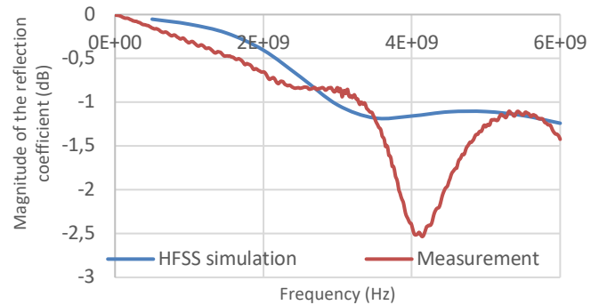
Fig 2. Simulated and measured magnitude of the reflection coefficient in the air
