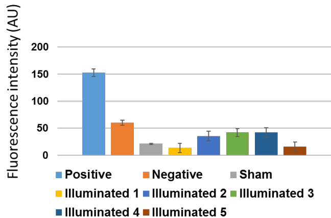
Fig. 3. Fluorescence intensity quantification after propidium iodide (PI) intake following five minutes RF-exposure (in CW mode) of HCT-116 multicellular spheroids.
