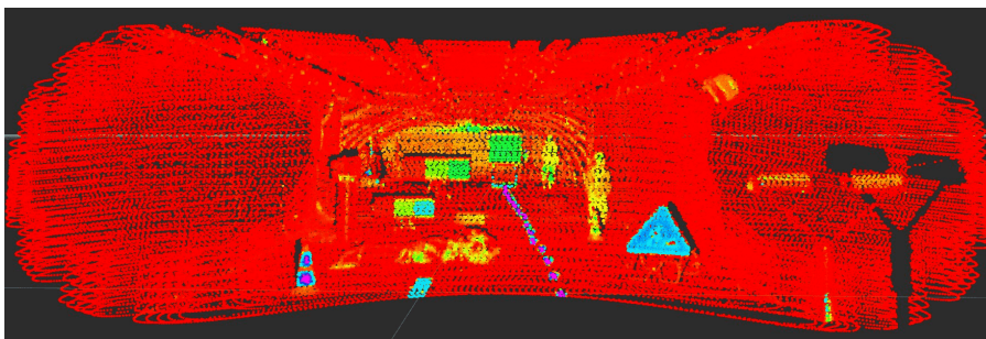
(b) Livox Horizon, accumulated scans, colored by intensity
