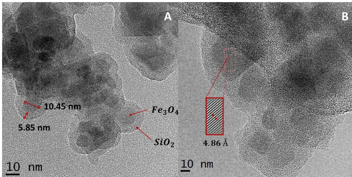
Fig. 4 HR-TEM images of \text{Fe}_3\text{O}_4@SiO_2 . A) Magnetic cores were measured with an average size of 10.45 nm and silica shells with 5.85 nm of thickness. B) Interplanar space of magnetite obtained with HR-TEM at 4.86 Å.
