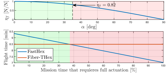
Fig. 5. Top: Nominal efficiency of the FAST-Hex depending on the tilting angle \alpha based on the efficiency index presented in (13). The index is computed for horizontal hovering ( \mathbf{R}_B = I_{3 \times 3} ) condition. For the maximum tilting angle \alpha = 35^\circ the efficiency drops to 0.82, meaning that 18% of the generated forces are “wasted” as internal forces. Bottom: Comparison of maximum flight time given the percentage of the mission that requires full actuation ( \alpha = 35^\circ ) for the FAST-Hex and the Fiber-THex [26], a fixed tilted hexarotor. If the mission profile requires less than 37% of the time full actuation (e.g., during taxi flights) then the FAST-Hex flight time is longer.
