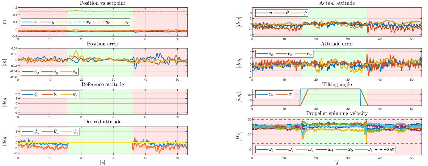
Fig. 9. Plots of Experiment 1 - left column from top to bottom: 1) Actual vs reference position; 2) Position tracking error; 3) Reference attitude depicted in Euler angles; 4) Desired attitude depicted in Euler angles. Right column from top to bottom: 5) Actual attitude depicted in Euler angles; 6) Attitude tracking error; 7) Reference and actual tilting angle; 8) Actual propeller spinning velocity. While the FAST-Hex is under-actuated the plots are highlighted in red. On the other hand, during full actuation the plots are highlighted in green.
