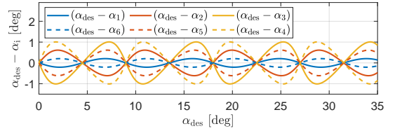
Fig. 4. Error between desired \alpha_{des} and actual tilting angle \alpha_i for the FAST-Hex for all six propellers. The absolute peak divergence is approximately 1^\circ . Therefore it has been decided not to consider it in the control design but to treat it as disturbance.
