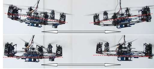
Fig. 10. Time-lapse pictures of the FAST-Hex during Experiment 2-a: Top: While being in UDT-configuration (tilting angle is zero) the platform cannot generate horizontal forces and the controller needs to adapt the attitude trajectory to be able to track the position trajectory. Bottom: With tilted propellers, the FAST-Hex is able to generate lateral forces and the platform can track independent position and attitude trajectories (depending on the actuation constraints) and therefore remain horizontal while traversing laterally.
