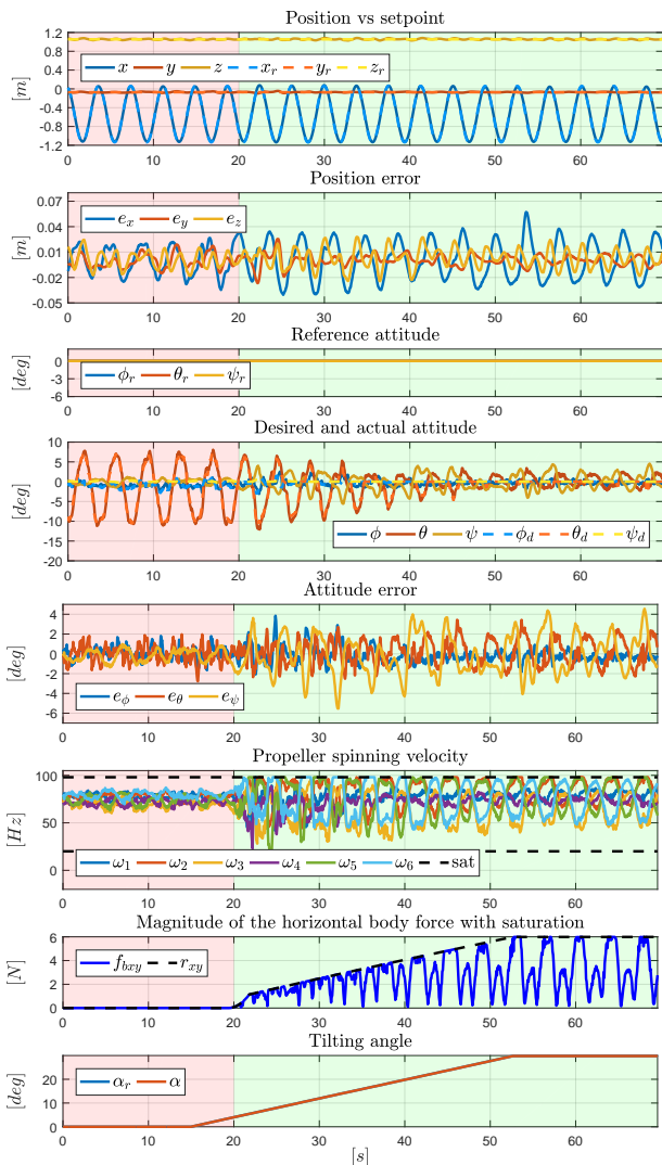
Fig. 11. Plots of Experiment 2-a - from top to bottom. 1) Actual vs reference position; 2) Position tracking error; 3) Reference attitude depicted in Euler angles; 4) Desired and actual attitude depicted in Euler angles; 5) Attitude tracking error; 6) Actual propeller spinning velocity; 7) Maximum and actual lateral force; 8) Reference and actual tilting angle. While the FAST-Hex is under-actuated, the plots are highlighted in red, during full actuation, the plots are highlighted in green.
