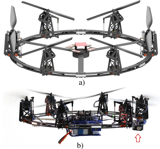
Fig. 1. a) CAD prototype of the FAST-Hex. All propellers are tilted in a synchronized manner by a single motor. b) Flying prototype with tilted propellers. The single servomotor for tilting all propellers is visible on the right bottom side of the ring structure and highlighted with an arrow.
