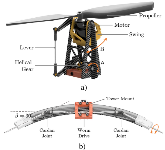
Fig. 2. a) CAD model of a single motor tower. A worm drive actuates the helical gear indicated by ‘A’ in the figure. The helical gear is rigidly connected on an axle, that is linked to a lever. The lever actuates a swing, which hosts the motor. The swing construction is used to rotate the the propeller close to its center. b) The complete MAV consists of six of the depicted elements. The top part of the ring is drawn transparent, allowing to see inside the ring structure. A single motor (not depicted in this figure) actuates the axes in the ring structure, that are connected with cardan joints. The direction of the worm drives is alternating, allowing the opposing rotation of neighboring motors.
