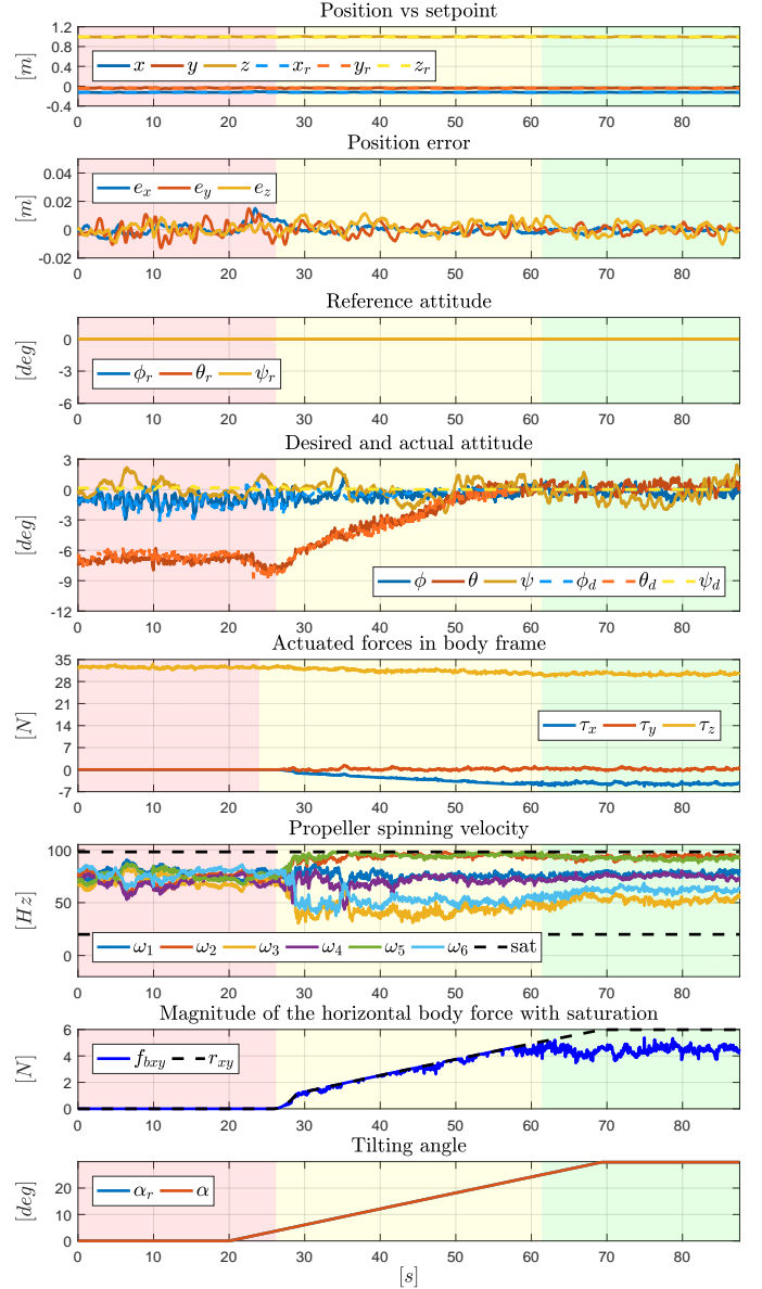
Fig. 1. Plots of Experiment 3 - from top to bottom. 1) Actual vs reference position; 2) Position tracking error; 3) Reference attitude depicted in Euler angles; 4) Desired and actual attitude depicted in Euler angles; 5) Actuated forces in body frame; 6) Actual propeller spinning velocity; 7) Maximum and actual lateral force; 8) Reference and actual tilting angle. While the FAST-Hex is under-actuated, the plots are highlighted in red, during full actuation, the plots are highlighted in green.
