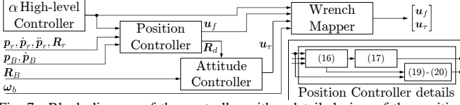
Fig. 7. Block diagram of the controller with a detailed view of the position controller including references to equations.
