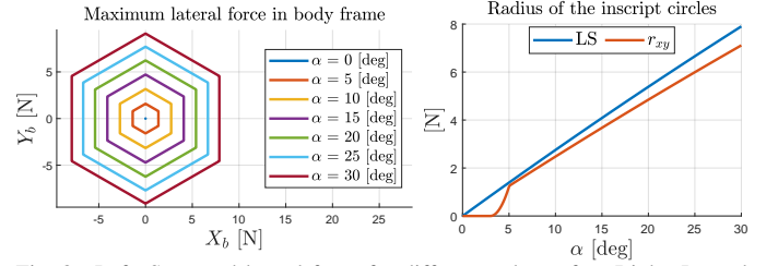
Fig. 8. Left: Saturated lateral force for different values of \alpha . Right: Lateral force saturation function.
