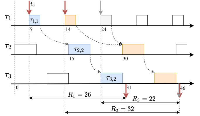
Fig. 1. Task chain run-time example with \tau_1 \rightarrow \tau_2 \rightarrow \tau_3
