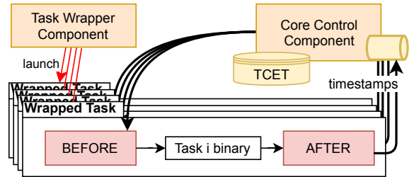
Fig. 4. Monitoring & Control Agent Architecture
