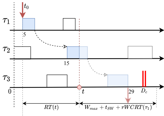
Fig. 2. active Task Chain Execution Trace with computed anticipation example
