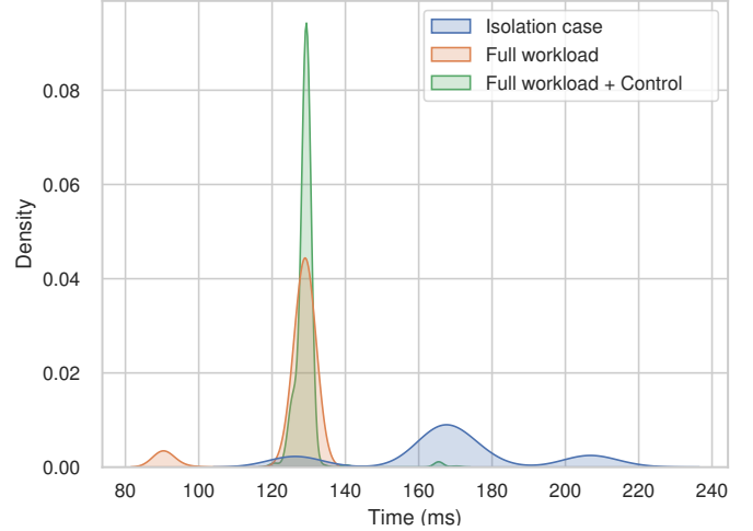
Fig. 7. Task Chain response time profile from steps ③, ⑥, ⑦
