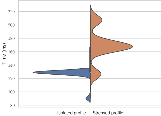
Fig. 6. Task chain end-to-end rWCRT distributions
