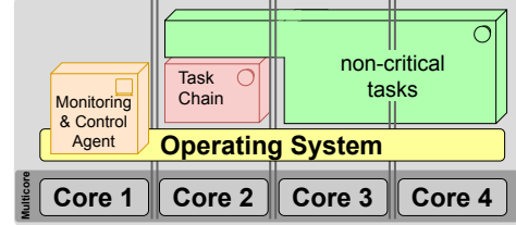
Fig. 3. Monitoring & Control Agent basic concept
