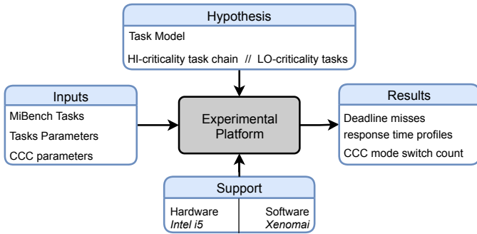
Fig. 5. Experimental Platform structure
