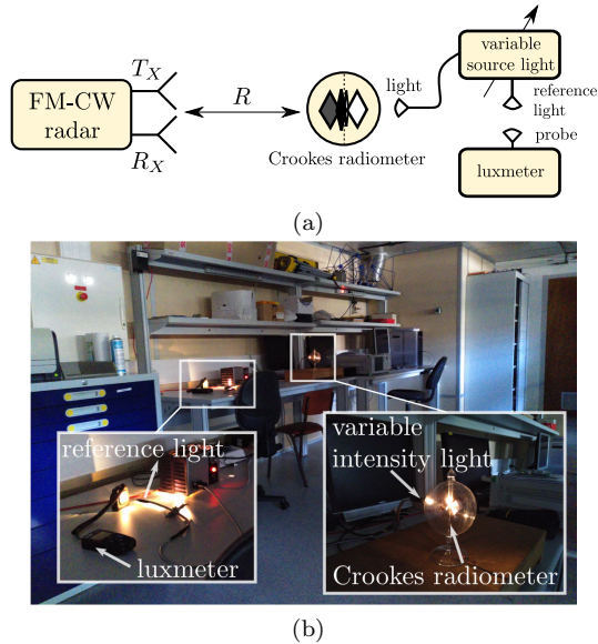
Figure 4: (a) Schematic of the experimental setup. (b) Second scenario where the Crookes radiometer is at a distance of 3.5m from the radar in a room of our Laboratory.
