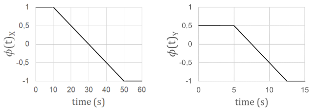
(a) Plot of \phi(t)_X of the sub-task X lasting 60 seconds, with SD_X = 10sec , V_X = 0.5 and \alpha = 1 (b) Plot of \phi(t)_Y of the sub-task Y lasting 15 seconds, with SD_Y = 5sec , V_Y = 1 and \alpha = 0.5
