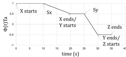
(c) Plot of \Phi(t)_{T_a} for a task composed of a sequence of three subtasks X, Y, Z : the duration of X exceeded SD_X = 10s and reached 20s , the duration of Y exceeded SD_Y = 5s and reached 10s , finally the duration of Z was less than SD_Z = 10s
