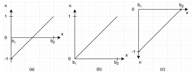
Fig. 11: (a), (b) and (c) respectively represent the min-max normalization functions (7), (8) and (9)
