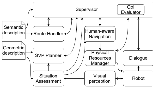
Fig. 5: The general architecture of the system running the direction-giving task.
