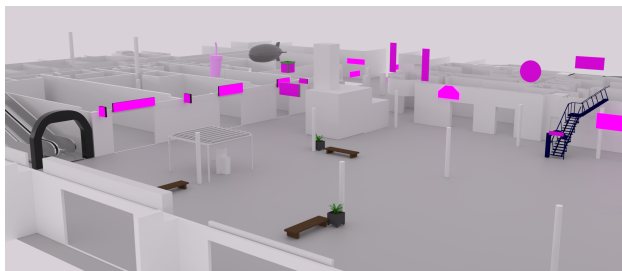
(a) 3D model of the Ideapark mall in Finland. The pink elements are storefronts.
