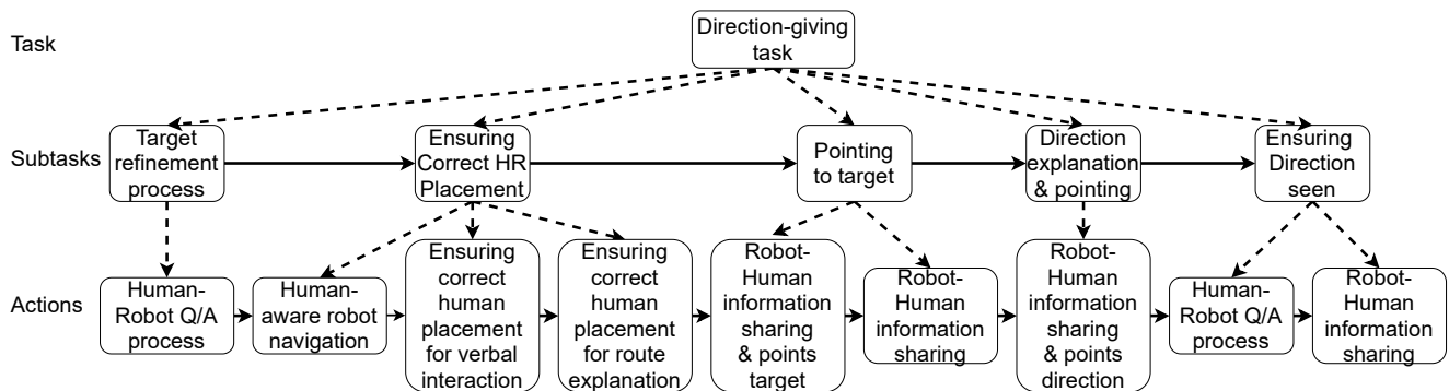
Fig. 8: The representation of the direction-giving task as a hierarchical task network with task, subtasks and actions levels. All the horizontal arrows are sequential links and the rest are decomposition ones.
