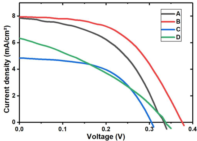
Fig. 6. J - V characteristics of 1 \text{ cm}^2 InGaAsN solar cells measured at 25^\circ\text{C} under \text{AM0} > 870 nm light.
