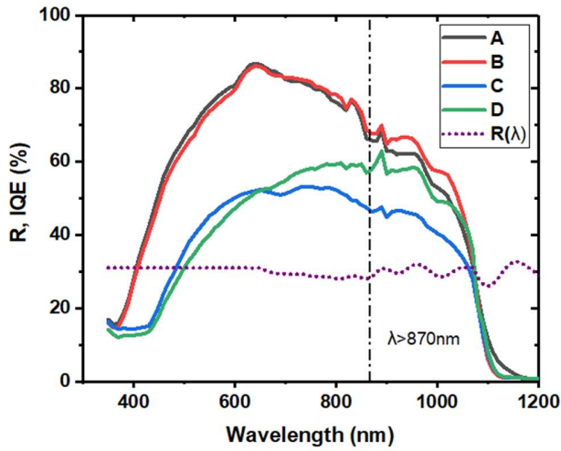
Fig. 5. Internal quantum efficiency and reflectance spectra of 0.25 \text{ cm}^2 InGaAsN solar cells.
