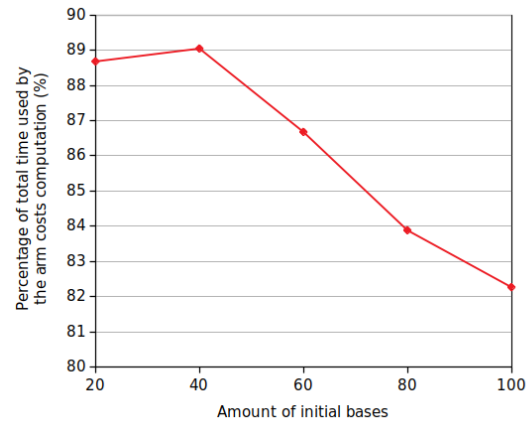
(b) Evolution of the percentage of total time used by the evaluation of the arm costs with the amount of initial base poses
