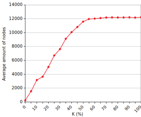
(a) Evolution of the amount of nodes with K
