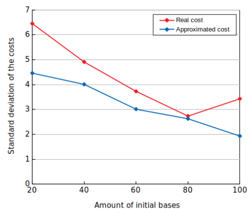
(b) Evolution of the standard deviation with the amount of initial base poses
