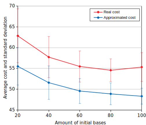
(a) Evolution of the costs and their deviation with the amount of initial base poses
