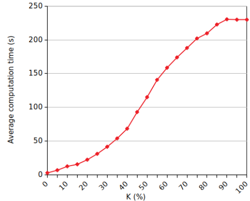
(b) Evolution of the computation time with K
