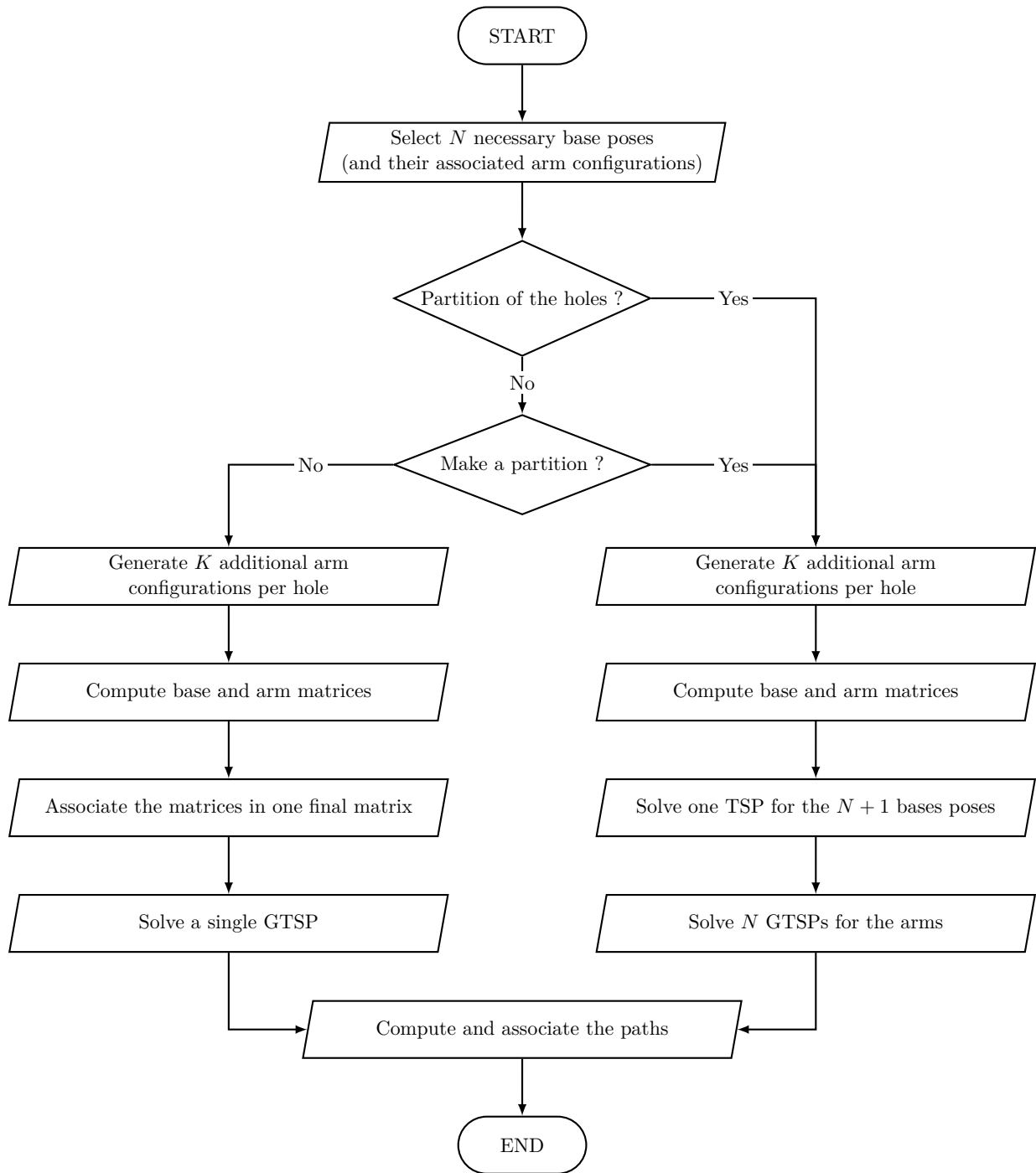
Figure 5.11: General principle of the approach involving the generation of additional arm configurations
