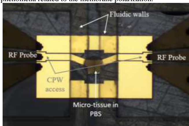
Fig. 1. Photography of the microwave sensor adapted to microtissue
