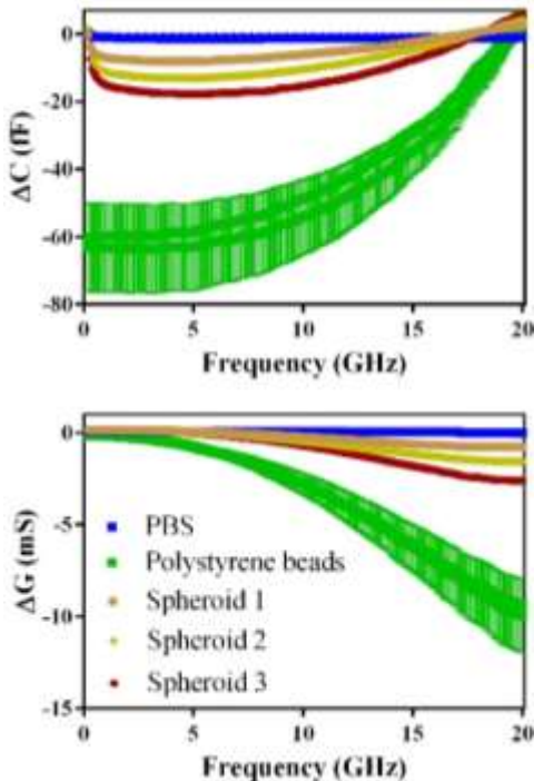
Fig. 4. Measured contrasts spectra obtained with the chosen reference fluid (PBS), polystyrene beads and fixed spheroids. Spheroid diameters are 262, 266
