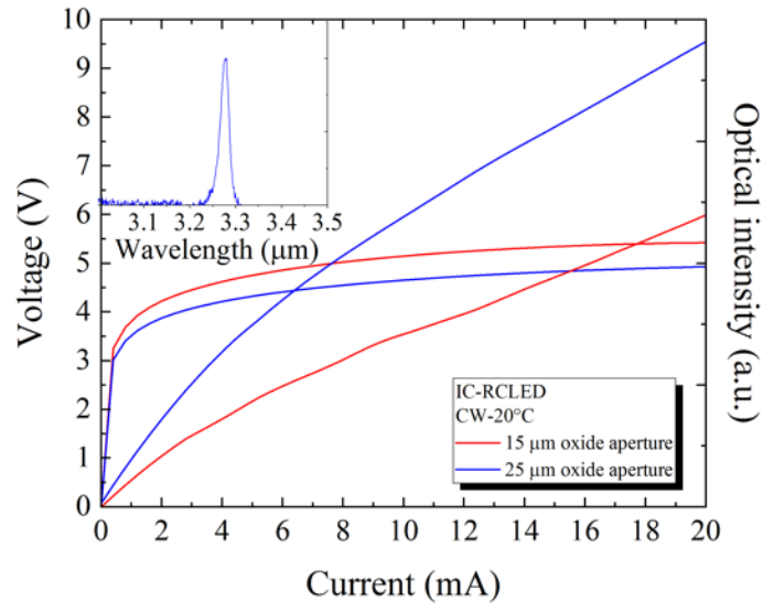
Fig. 1. L-I-V of IC-RCLED in CW at 20°C with AlOx aperture of 15 μm (red) and 25 μm (blue). Insert: Spectrum taken in CW at 20°C of the IC-RCLED with aperture of 25 μm.
