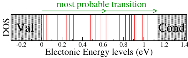
Fig. 2: Si band gap and the localised defect states (red) induced by the cluster 14-I (using DFT-HSE). Arrows indicate the closest to mid-gap transition.
