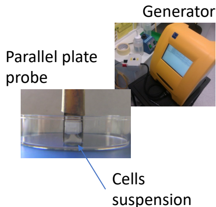
Figure 3. Electroporation setup.
