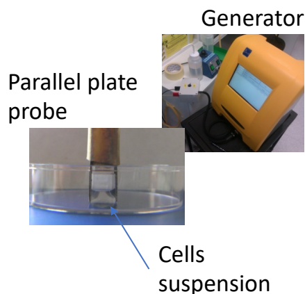
Figure 3. Electroporation setup.
