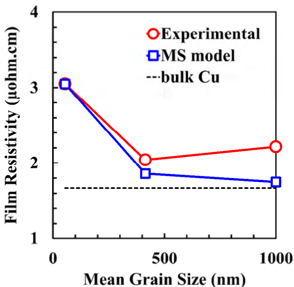
Fig. 4. Experimental and theoretical (based on the Mayadas-Shatzkes (MS) model) film resistivity of the non-annealed and annealed samples.
