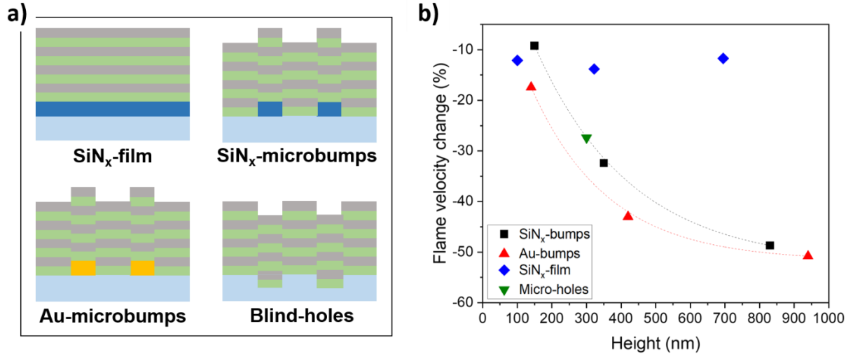
Figure 4. (a) Cross-sectional schematics of the different sample configurations. (b) Flame velocity change of Al/CuO multilayers deposited on the different configurations of substrates described in (a): SiN x film (blue), Au microbumps (red), SiN x microbumps (black), and blind microholes (green). Depending on the configuration, the x-axis represents the microbump height, the SiN x film thickness or the blind-hole depth.
