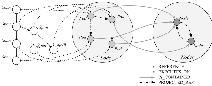
Fig. 4. Hierarchical Graph Representation.
