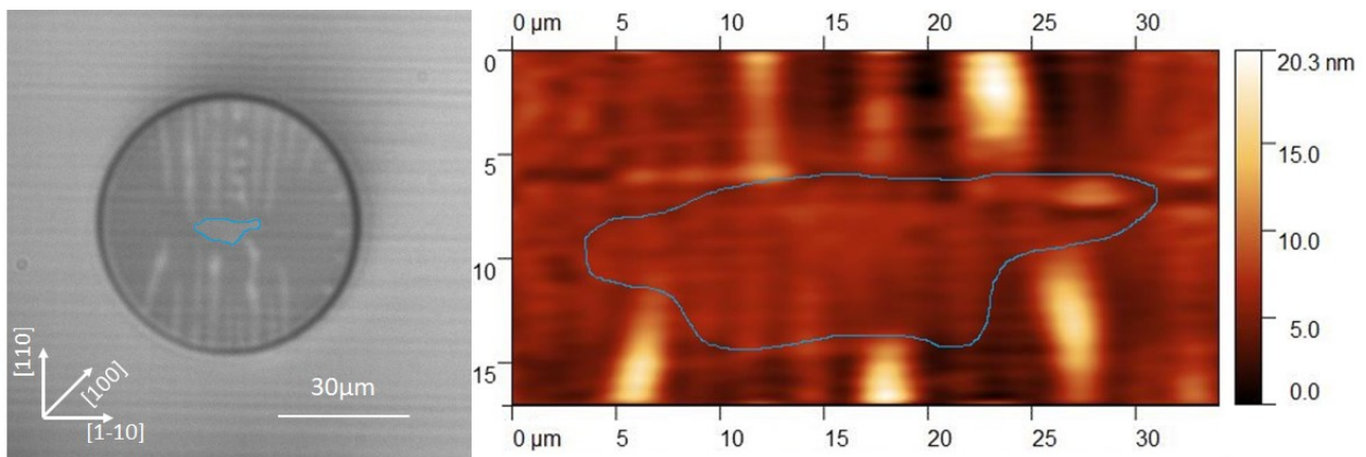
Fig. 11. Infrared image left and atomic force microscope surface profile of an oxidized AlAsSb 13.4% 60-μm-diameter with the oxide aperture contours highlighted in blue. The oxidation conditions are 420°C & 500 mbar for 20 min.
