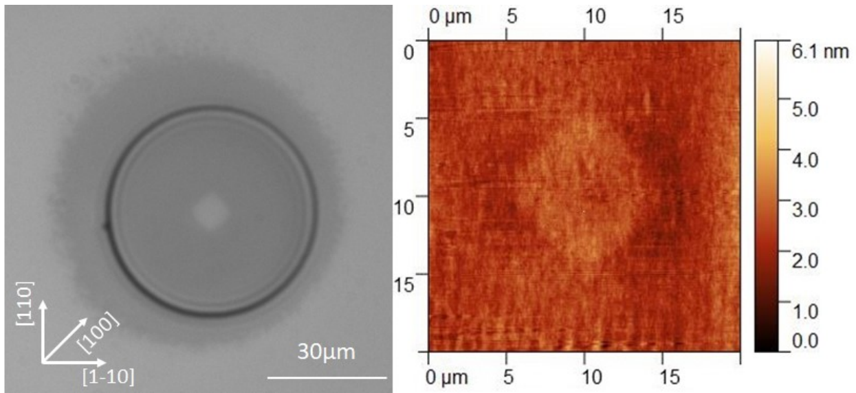
Fig. 3. Infrared image (left) of a 52 \mu\text{m} -diameter circular mesa embedding an AlAsSb 6.9% layer oxidized at 380°C – 500 mbar for 63min and its atomic force microscope surface profile (right).
