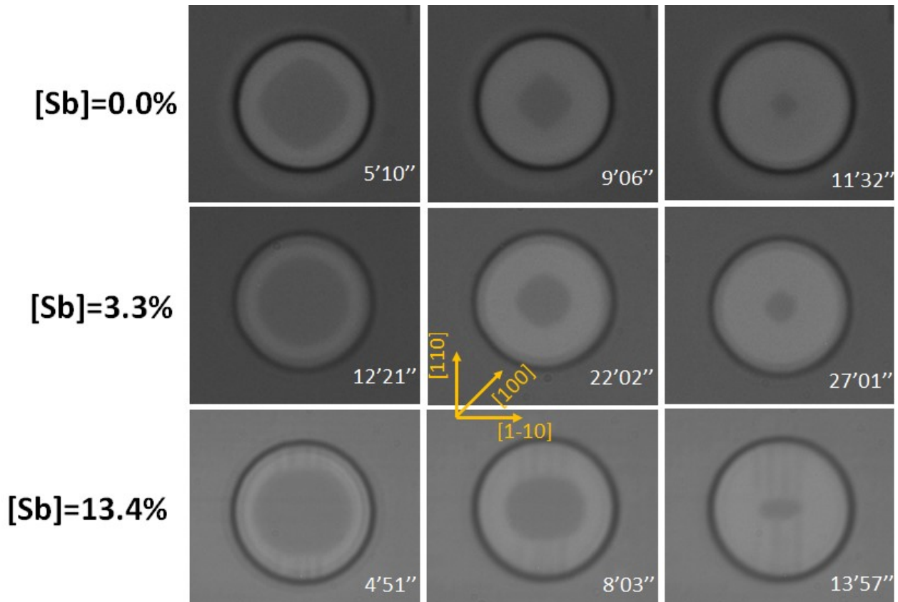
Fig. 2. Infrared microscopy images measured in-situ during the oxidation (at 420°C, 500 mbar) of 42 μm-diameter circular mesas of \text{AlAsSb} with different \text{Sb} concentration.
