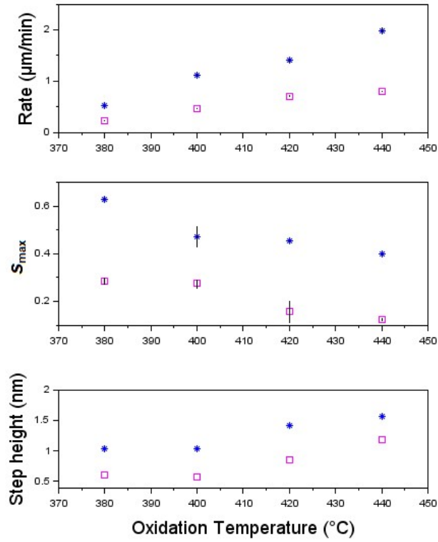
Fig. 5. Temperature dependence of ALAs (blue) AlAs_{0.967}Sb_{0.033} (pink) oxidation: rate, square fraction of the aperture shape and semiconductor-to-oxide step height measured from circular mesas. Measurement error bars are indicated when relevant.
