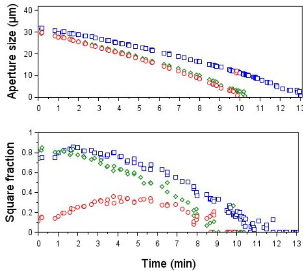
Fig. 4. Time dependence of the oxidation (420°C – 500 mbar) of AlAs from 42μm etched mesa whose shape is a circle (red), a (110)-oriented (blue) square or a (100)-oriented (green) square. The start time t=0 min is taken here as the time when the aperture of the (110)-oriented square can be distinguished from its etched mesa contour.
