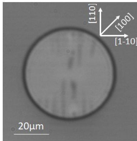
Fig. 10. Typical strain-induced drumhead pattern observed upon full oxidation (at 420°C & 500 mbar for 20 min) of AlAsSb 13.4% -containing 52-μm-diameter circular mesa.
