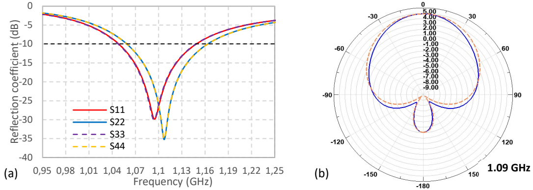
Figure 4: (a) Simulated reflection coefficient at each port of the antenna; (b) the radiation pattern of the PIFA antenna array in two vertical planes: xOz/\varphi=0^\circ (blue solid line) and yOz/\varphi= 90^\circ (orange dash line).
