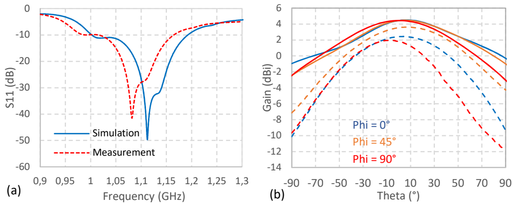
Figure 10: (a) Measured (dashed line) and simulated (continuous line) reflection coefficient at the input of the feed port of the PIFA array; (b) the simulated (continuous line) and measured (dashed line) gain for three vertical cut planes ( \varphi = 0^{\circ} , \varphi = 45^{\circ} and \varphi = 90^{\circ} ).
