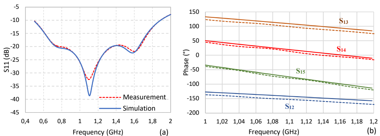
Figure 8: (a) Simulated (line) and measured (dashed line) of the reflection coefficient (at the input of the feed port); (b) The phase delay between port 1 and each of the others.
