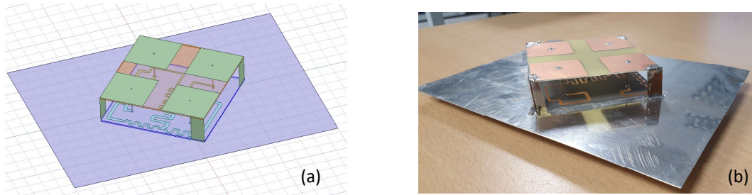
Figure 9: (a) Designed antenna on HFSS Software; (b) Photograph of the manufactured antenna.
