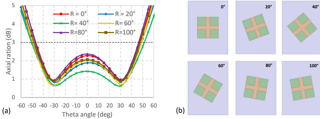
Figure 5: (a) Variation of the axial ratio as function of the antenna rotation angle at \varphi=0^\circ and 1.09 GHz; (b) antenna rotation angle with the respect to the reflector.
