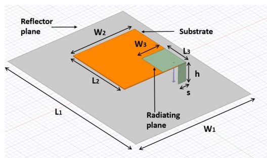
Figure 1: Configuration of the antenna with single PIFA.
