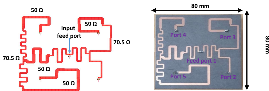
Figure 7: Layout and photograph of the fabricated quadrature feed network.
