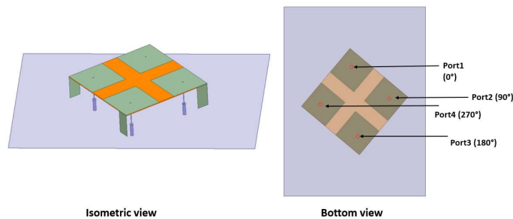
Figure 3: Isometric and bottom view of the array PIFA antenna.
