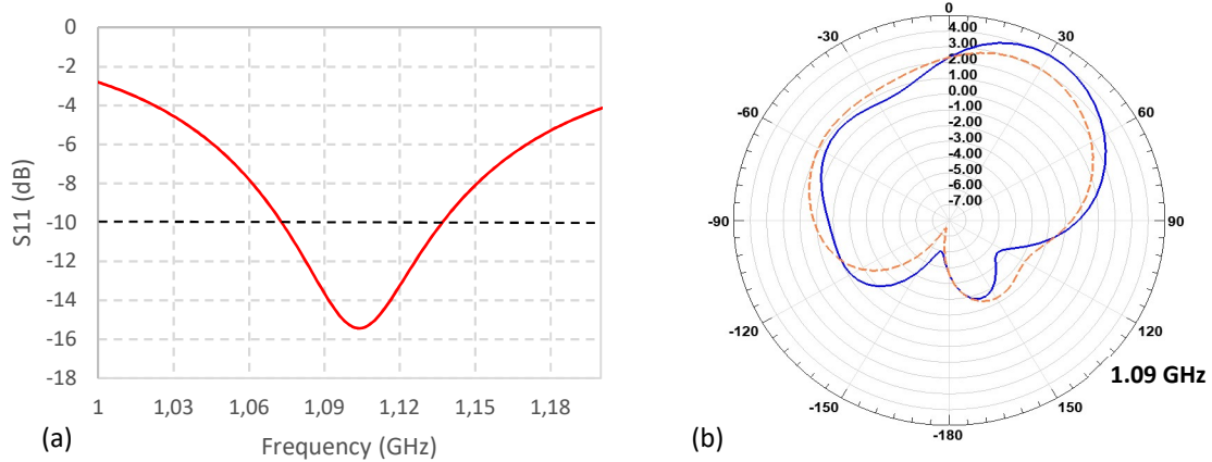
Figure 2: (a) Simulated reflection coefficient and (b) radiated pattern of a single PIFA antenna ( xOz/\varphi=0^\circ cut -blue solid line- and yOz/\varphi=90^\circ -orange dash line-).
