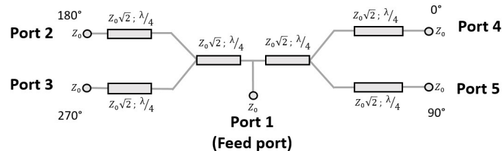
Figure 6: Circuit model of the feed network.
