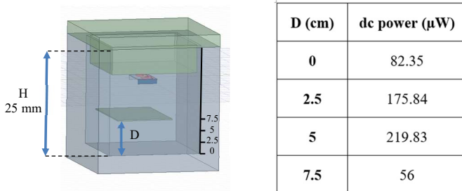
Figure 7. dc power as function of the position of the rectenna (R2) inside the covered concrete cavity (top green part is the cover).
