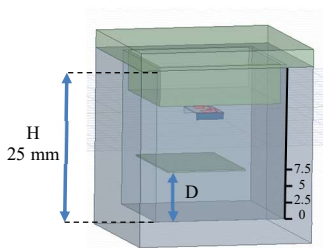
Figure 7. dc power as function of the position of the rectenna (R2) inside the covered concrete cavity (top green part is the cover).
