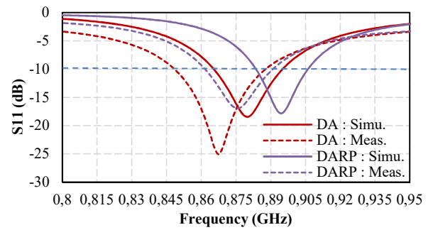
Figure 3. Comparison of the simulated and measured reflection coefficient of DA and DARP antennas.
