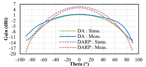
Figure 4. Simulated and measured radiation patterns (gain in dBi) of the DA and DARP antennas in the E-plane at 868 MHz.
