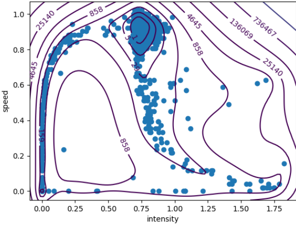
Fig. 4. Levelsets obtained from the Luggage Conveyor dataset for d = 6 . The levelset labelled as 858 captures the two main operating modes, the transitions and most of the points from the dragged mode.
