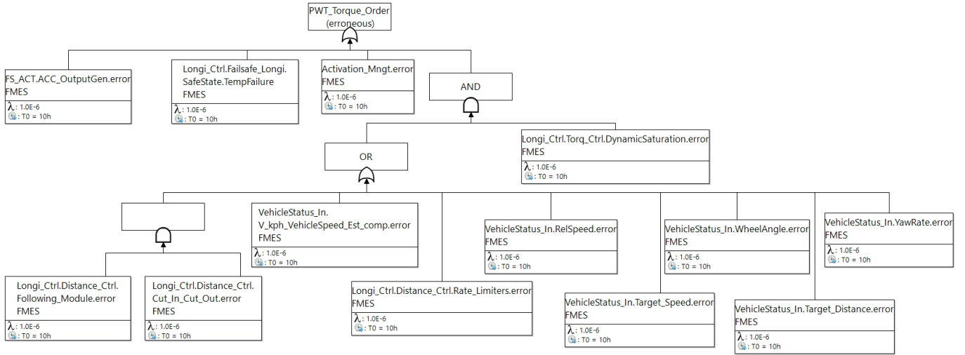
Figure 13. Fault tree
