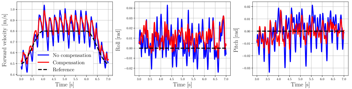
Fig. 4: The compensation of the contact forces reduces the oscillation in forward velocity, roll and pitch.
