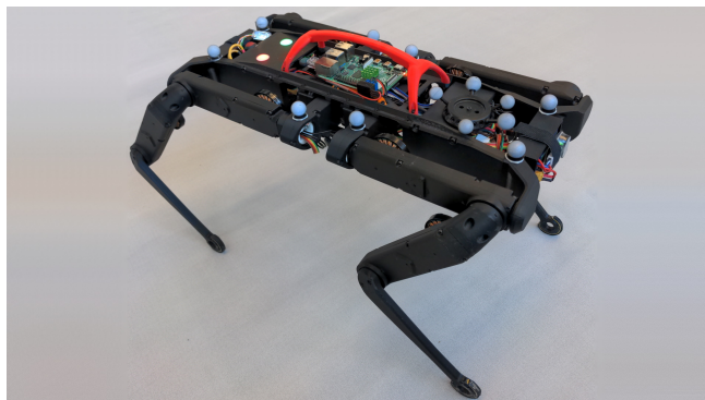
Fig. 1: Solo-12 quadruped powered with batteries. The whole control architecture can run on an on-board Raspberry Pi 4.
