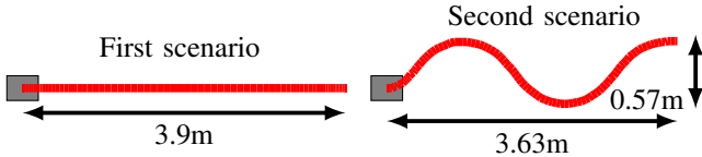
Fig. 8: Top view of the robot trajectory in the two considered scenarios obtained by integration of the reference velocity.
