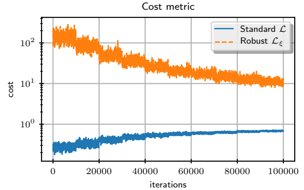
Fig. 4: Robust cost metric \mathcal{L}_\xi evolution trend during CMA-ES (orange curve). \mathcal{L}_\xi diminishes for each iteration of Alg. 1, while the standard cost \mathcal{L} increases (blue curve).
