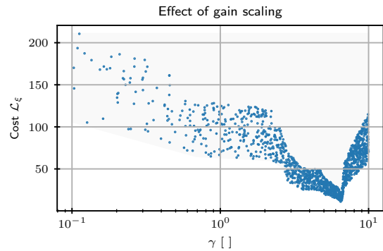
Fig. 9: Effect of the scaling \gamma with respect to the robust cost \mathcal{L}_\xi . Each dot represents an individual of the optimization. The presence of a minimum can be seen
