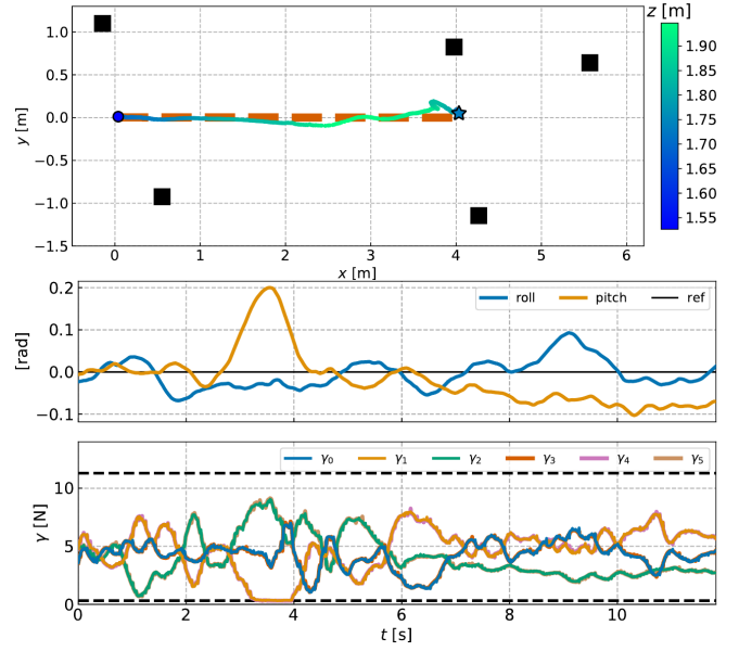
Fig. 3: Simulation with a tilted-propeller hexarotor and a down-facing camera. Above, the (x, y) trajectory using the same presentation as Fig. 2. Below, the roll/pitch angles of the tilted-propeller hexarotor, as well as the 6 propeller thrusts, over time.
