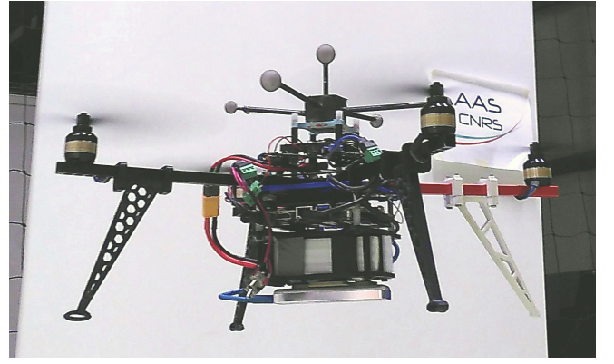
Fig. 1: Snapshot of the platform used in the reported experiment.
