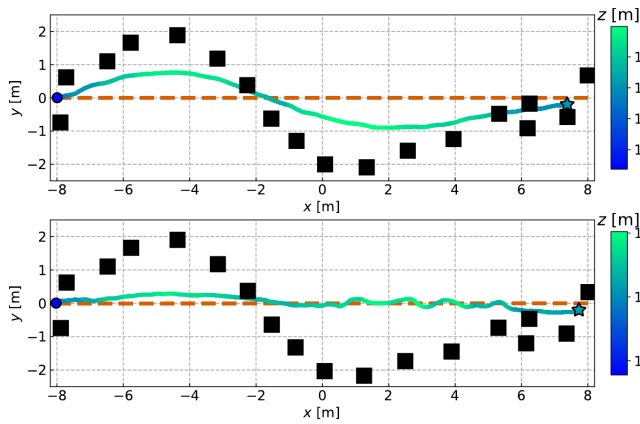
Fig. 4: Simulations using a quadrotor (top) and a tilted-propeller hexarotor (bottom). The same presentation as Fig. 2 is used. Both N-MPC are tuned with the same set of weights.
