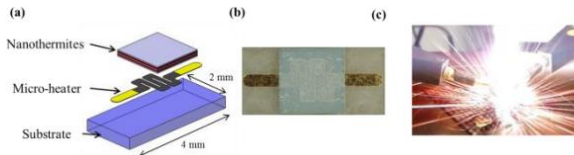
FIG. 5. (a) 3D schematic representation of a pyroMEMS; (b) photo of the pyroMEMS; (c) photo during the nanothermite reaction 27 .
