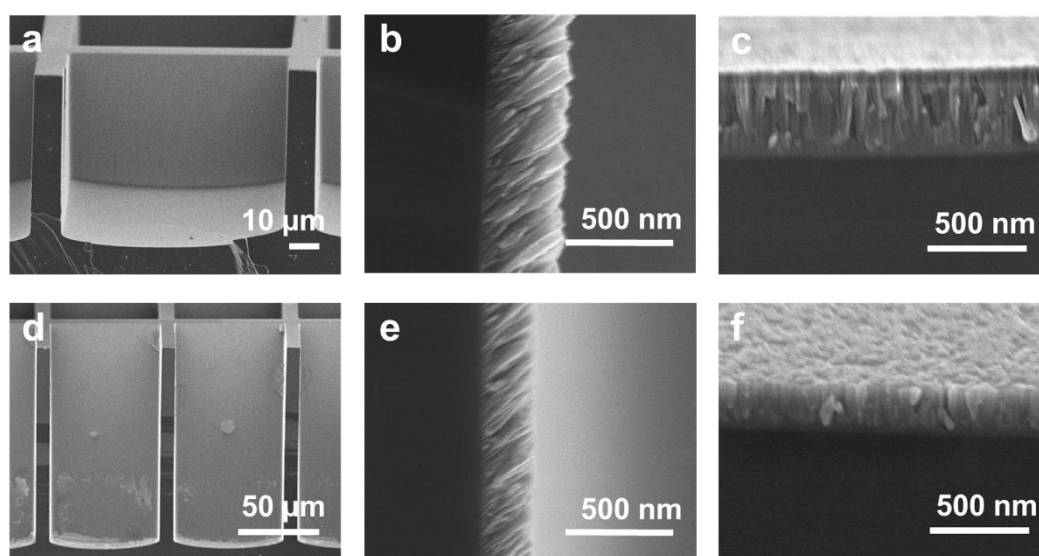
Figure 8. SEM cross-sectional images of the 3D photocatalyst composed of silicon microstructures and TiO 2 film, corresponding to samples A3-T2 (a-c) and A7-T2 (d-f) featuring AEFs of 3 and 7, respectively. Details of the compact TiO 2 layer at half-heights of the wall (b, e) and bottom of the microcavities (c, f).
