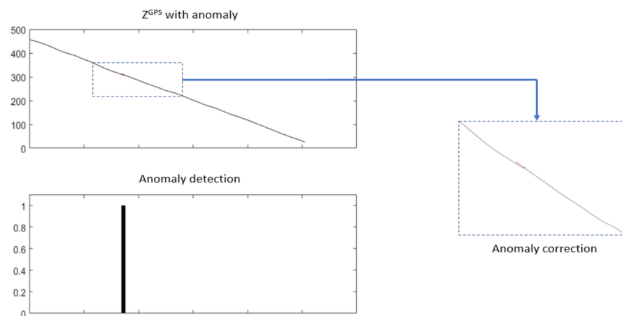
Figure 23. Anomaly detected and corrected using NADCA-L. The small anomaly appears in red.
